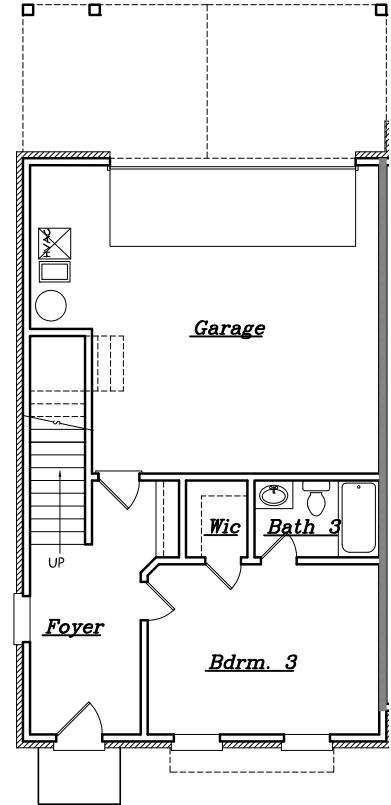
Terrace Level
